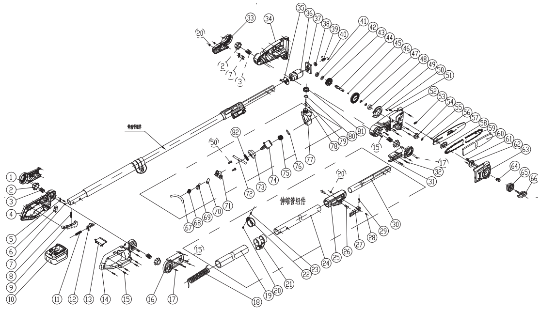
Exploded Drawing of Cordless pole saw RDP-SPS20 Art. No. 075708
